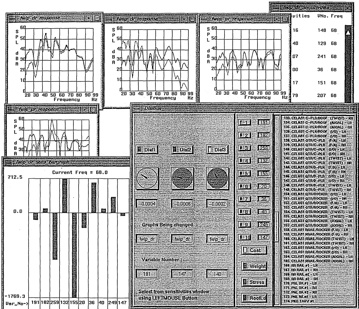
Figure 7: VISUAL INTERFACE SHOWING MULTIPLE GRAPHS, DIAL BOX INPUT AND SENSITIVITIES
