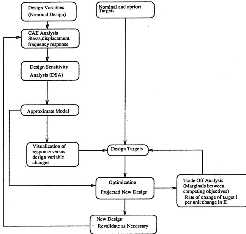
Figure 1: FLOW CHART FOR STRUCTURAL/ACOUSTIC ANALYSIS
