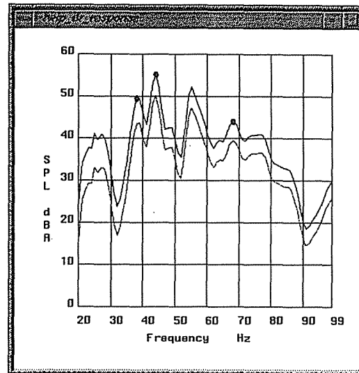
Figure 6: BASE LINE AND MODIFIED SPL
