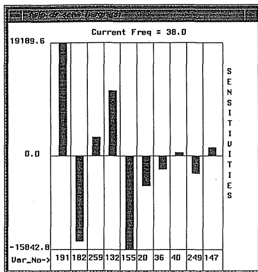
Figure 4: BAR GRAPH OF SENSITIVITIES AT PEAK FREQ. 38 Hz FOR THE fwip DRIVERS EAR CASE
