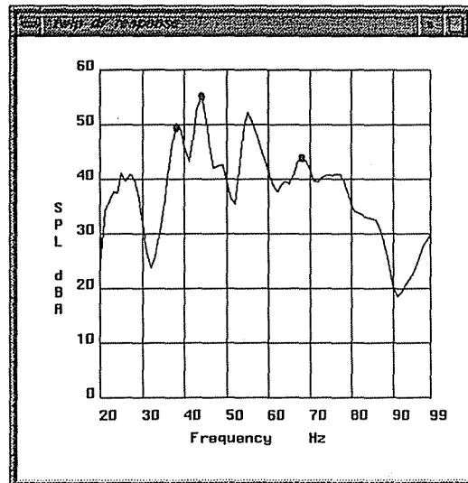
Figure 2: SPL AT THE DRIVERS EAR, FRONT WHEELS IN PHASE ( fwip ) CASE
