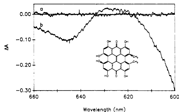
Figure 1. Transient absorption spectrum of hypericin in methanol at 20 °C using a charge-coupled device (Princeton Instruments 1152UV). \lambda_{\text{ex}} = 588 \text{ nm} . (a) Delay time of -20 ps between the pump and the probe pulse. This is the control experiment that demonstrates that the observed signal is due to the excitation or pump pulse. (b) "Zero" delay between pump and probe. Three distinct phenomena are observed. From lower wavelength to higher wavelength, they are (1) bleaching of the ground-state absorption of hypericin; (2) a new transient species whose absorbance can be clearly seen at \sim 630 \text{ nm} ; and (3) a transmission increase in a region where there is no ground-state absorbance (this corresponds to stimulated emission from excited-state hypericin). The short-lived absorbance at 630 nm is attributed to formation of a species with a protonated carbonyl (see text). This assignment is based on our result that the hypericin along with no hydroxyl groups, mesonaphthobianthrone, exhibits essentially no fluorescence in the aprotic solvent DMSO. In \text{H}_2\text{SO}_4 , however, its absorption and fluorescence spectra are nearly identical to those of hypericin.
