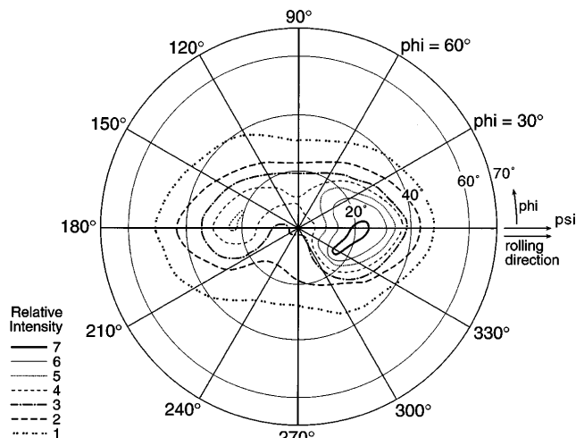
FIG. 4. Pole figure for the (0002) plane of the Sc phase rolled at 873 K to \eta = 4.2 .
