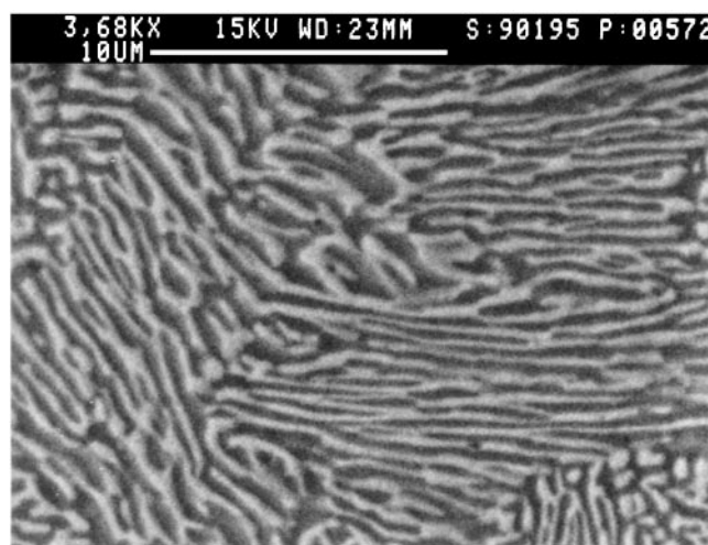
FIG. 1. Backscattered electron SEM image of the rapidly solidified eutectoid microstructure of as-cast 59Sc-41Ti specimen (unetched). Ti is light gray; Sc is dark gray.
