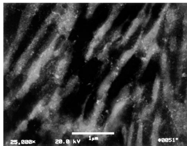
FIG. 2. Backscattered electron image of the 59Sc-41Ti specimen (unetched) after rolling at 873 K to \eta = 2.3 . Ti is light gray; Sc is dark gray. This cross section was cut showing the sample as viewed along the rolling direction.
