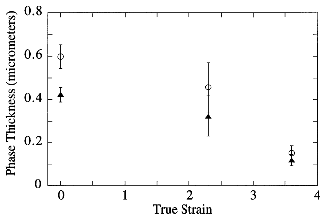
FIG. 3. Relation between phase size and deformation processed true strain. Open circles are Sc mean phase thickness; closed symbols are Ti mean phase thickness. Error bars indicate \pm one standard deviation from the mean value.
