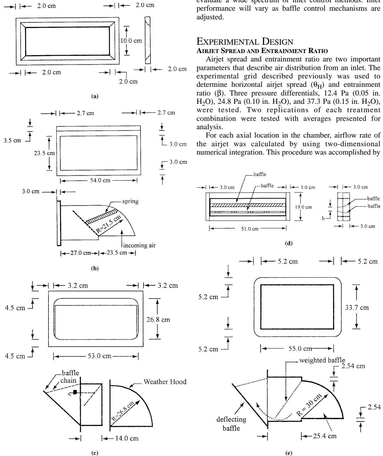
Figure 3—Wall inlets tested.
