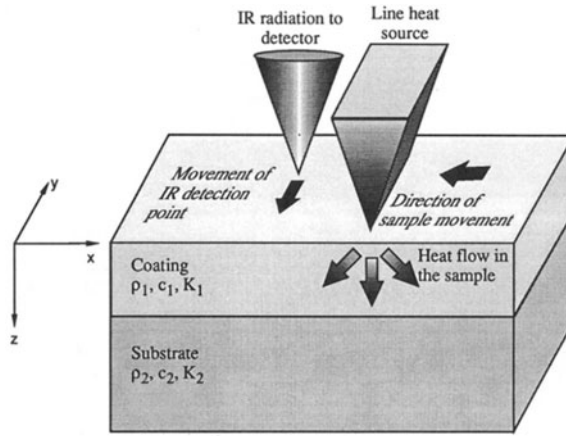
Figure 1. The measurement principle.
