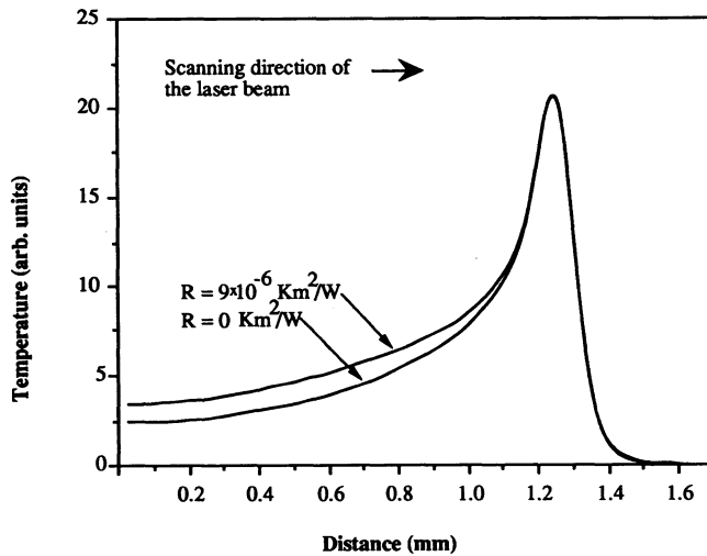
Figure 2. An example of the numerically computed temperature profiles along the x -axis when a line heat source parallel to the y -axis is moved to the positive x direction. The numeric values used in computations are: \rho_1 = 5210 \text{ kg/m}^3 , \rho_2 = 7860 \text{ kg/m}^3 , c_1 = 781 \text{ J/kgK} , c_2 = 450 \text{ J/kgK} , \kappa_1 = 10 \text{ W/Km} , and \kappa_2 = 10 \text{ W/Km} . The coating thickness is 200 \text{ }\mu\text{m} , the heating beam width is 200 \text{ }\mu\text{m} , and the scanning speed in the x direction is 5 \text{ cm/s} .
