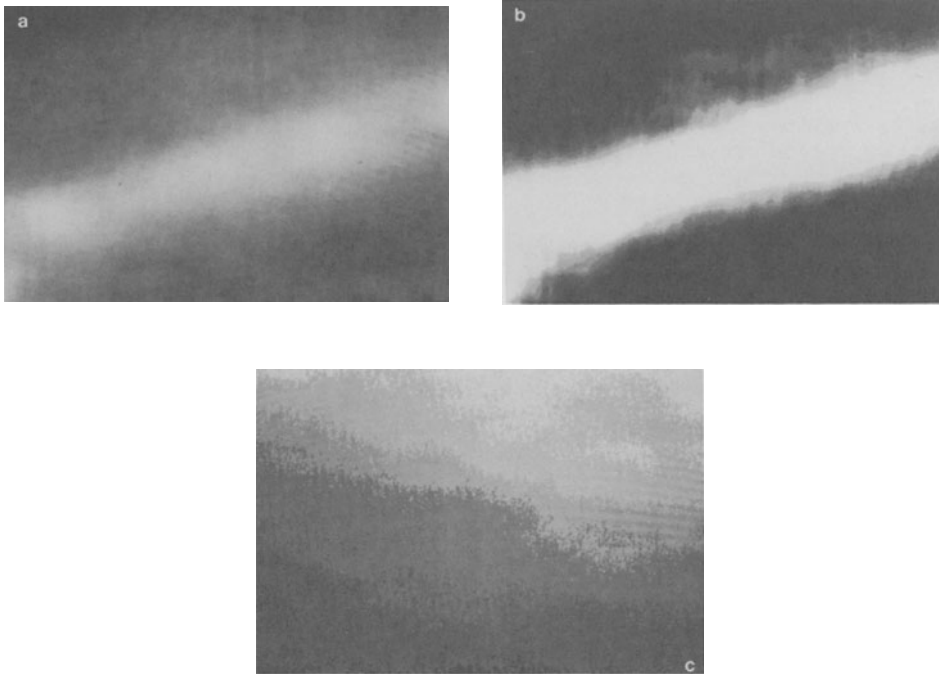
Figure 4. (a) The original and (b) the enhanced photothermal image of an adhesion defect in a plasma sprayed chromium oxide coating on steel substrate. (c) The optical image of the measured area. The size of the measured area is 4 \times 5 \text{ mm}^2 .
