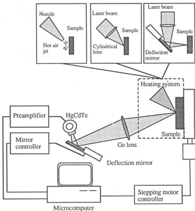
Figure 3. A diagram of the measurement system.
