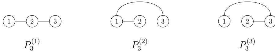
Figure 1.2 The three nonisomorphic labelings of P_3 .
