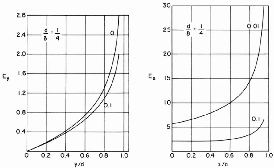
Fig. 3. Electric fields \text{Re}E_y(y) and \text{Re}E_x(x) at the surfaces of an open crack for d/\delta=1/4 . The numbers by the curves indicate the ratio of the width to the skin depth, 2a/\delta .
